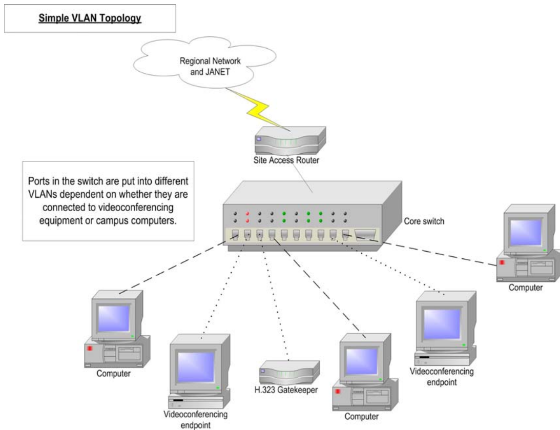
Figure 8: Simple VLANs.
