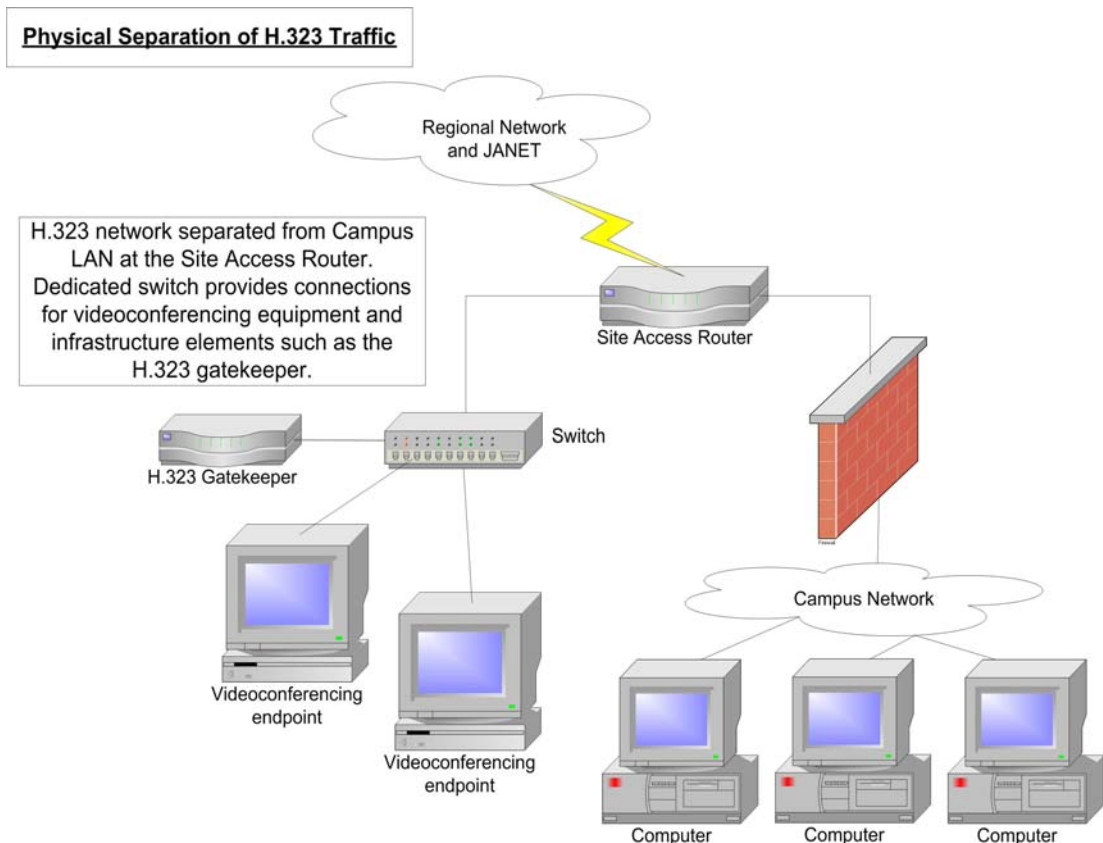
Figure 6: Physical separation.
