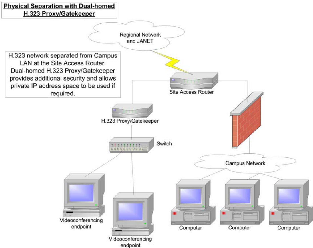
Figure 7: Dual-homed gatekeeper/proxy.
